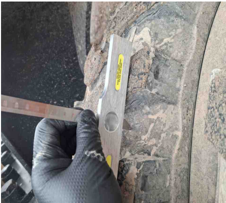
Wheel Position: B2 - Tread Depth Gauge(Removed)
