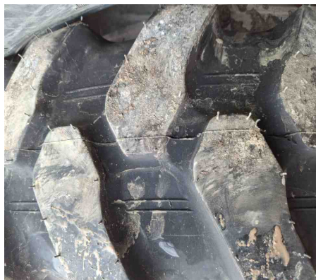
Wheel Position: B2 - Tread After
