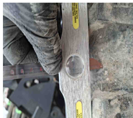
Wheel Position: A2 - Tread Depth Gauge
