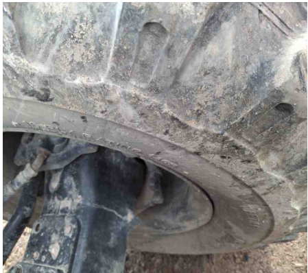
Wheel Position: A2 - Sidewall After
