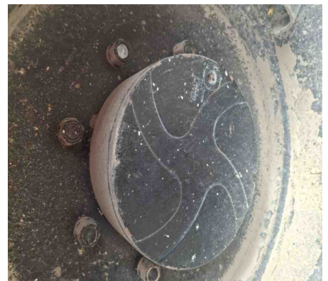
Wheel Position: A1 - Wheel Nut After
